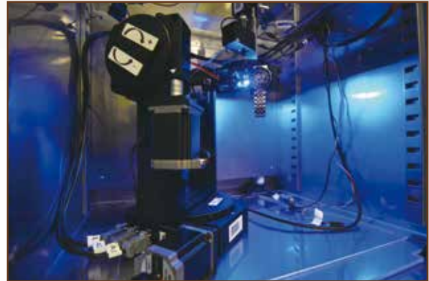
Hong Kong's first chronometer test equipment for mechanical movements and electronic/quartz movements. It ensures the accuracy of watches by referencing the Coordinated Universal Time against atomic clocks of satellites via GPS.
